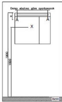
Upper Cabinet Suspension Distance = 1900-X
