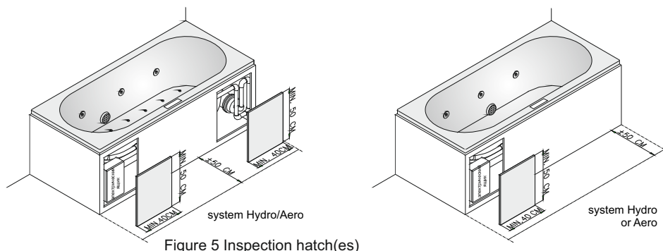
Figure 5 Inspection hatch(es)
